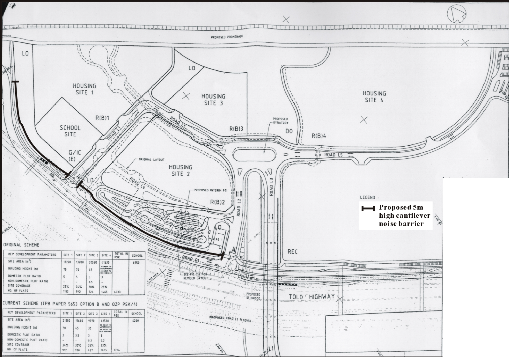
Figure 2 Location of Noise Barriers along Road D1 for Pak Shek Kok Development
