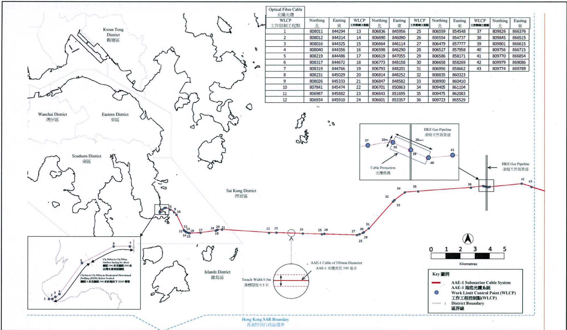
Figure 1: The landing site and the route alignment of the cable 圖 1: 光纜系統登岸地點及海上路線
