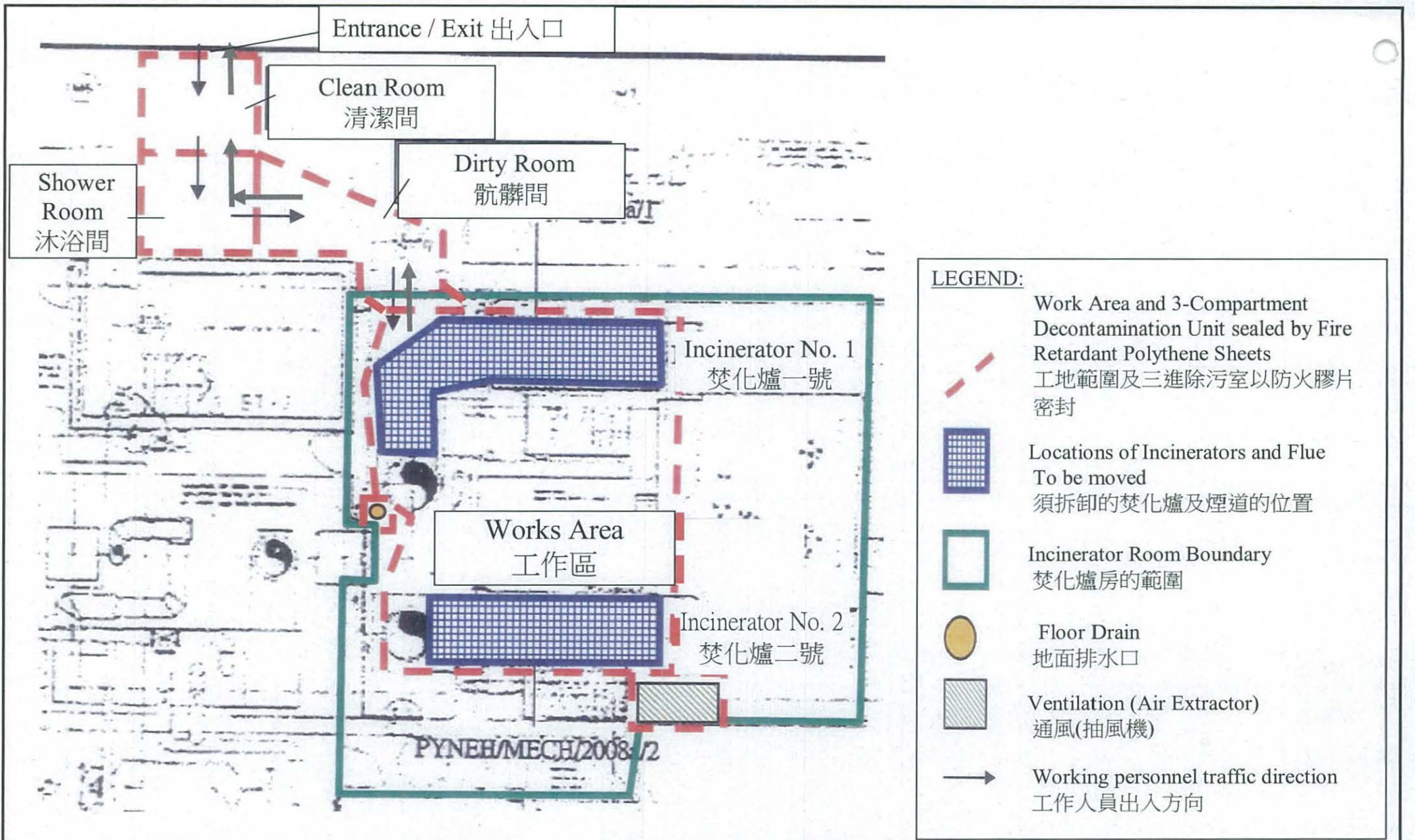
Figure 2: Floor Plan of the Works Area
