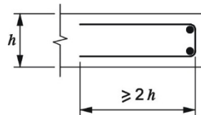
Figure 9.4 - Edge reinforcement for a slab
