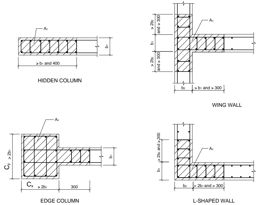
(b) Type 3 confined boundary elements
