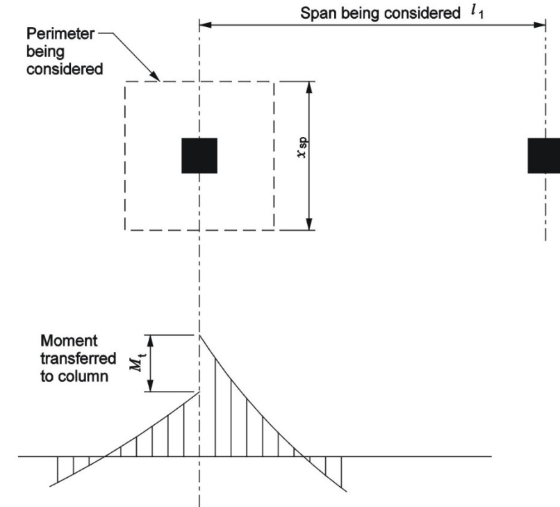
a) Bending moments diagram for load case being considered
