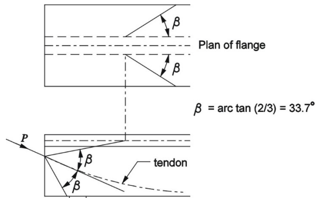
Figure 8.12 - Dispersion of prestress
